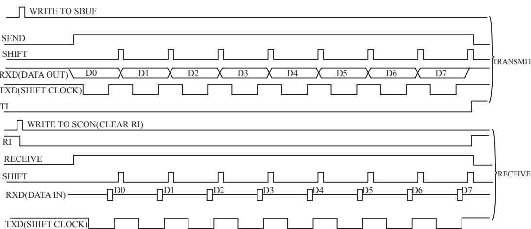
Serial Port Mode 0
