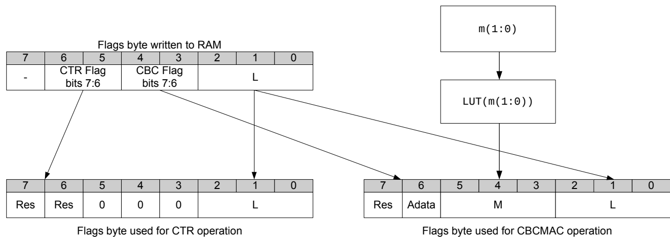
Figure 35: Security flags
